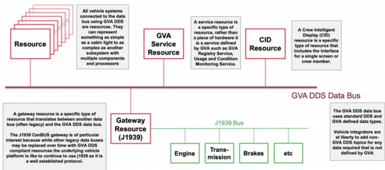
Figure 7: GVA based vehicle data architecture
