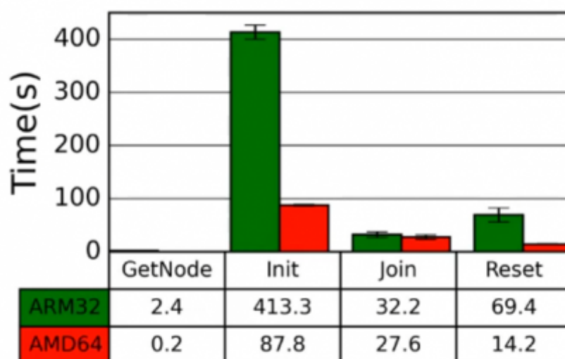
Fig2. kubectrl operation cost comparison
