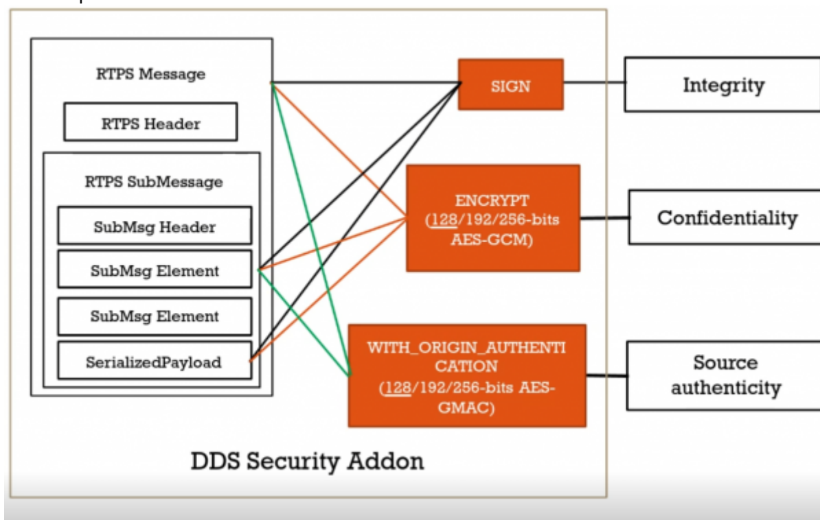
Figure 8: This illustrates the DDS Security Plugin
