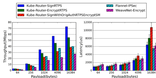
Fig7. Performance comparison of security implementations on application-layer(DDS Security plugin) and network-layer(Flannel-IPSec, WeaveNet-Encrypt). Communication pattern: 1pub-1sub . Reliability: enabled, Batching: disabled. Test period: 120 seconds.
